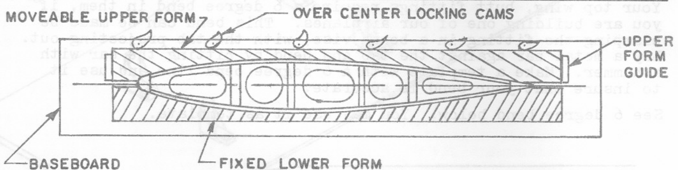
TYP. JIG FOR THIN WEB/CAPSTRIP TYPE RIBS
